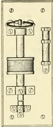
Fig. 125. Typical Form of Lightning Arrester
